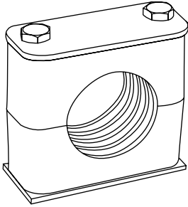
Standard Series – for outside diameters from 1/4" to 2". Clamp material: Polypropylene
