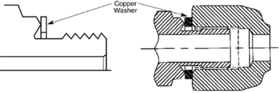
Figure 75 BSPP
