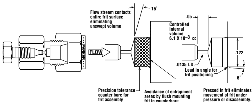
Figure 72 Press In Frit Design
