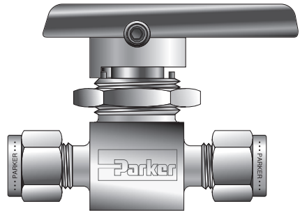
Model shown: 4A-MB6LPFA-SSP Two-Way In-Line
