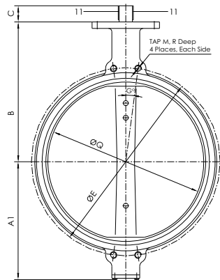
Front View BF 75 > Wafer Style
