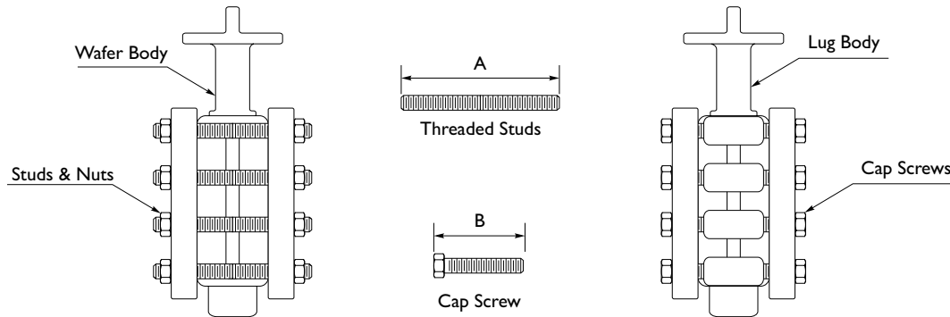
WAFFER STYLE FLANGE BOLT DATA (1)
